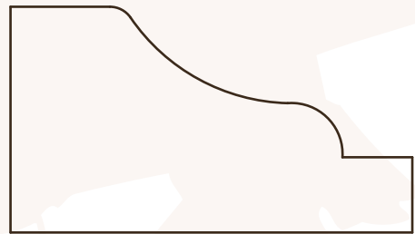
COLONIAL RAKE 2"x1-1/8" P
