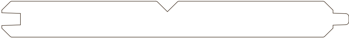
C-68 3/4"x7-1/4"
