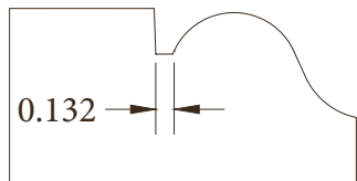
C-69 1-1/4"x2-1/2"
