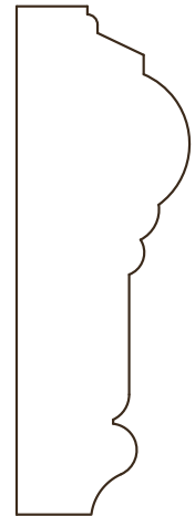
F-12 1"x3-1/8" O,B,P
