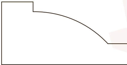
STANDARD RAKE 2-1/4"x1-1/8" P
