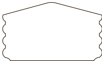
PORCH RAIL 1-1/2"x2-1/2" P
